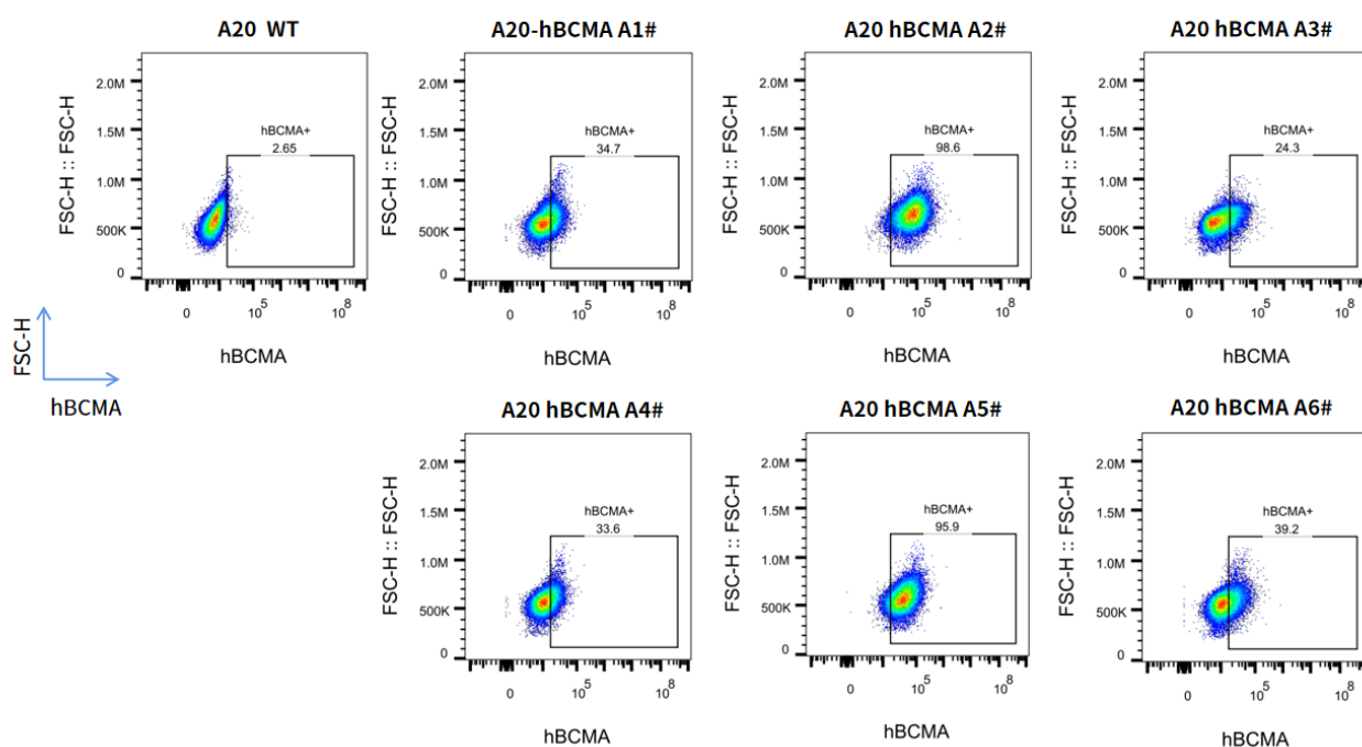
Fig1. hBCMA expression on in vitro cultured cells of A20-hBCMA.
