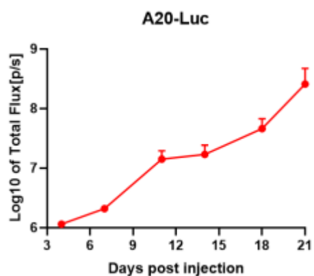
Figure 1. Luciferase activity assay of A20-Luc cell line
