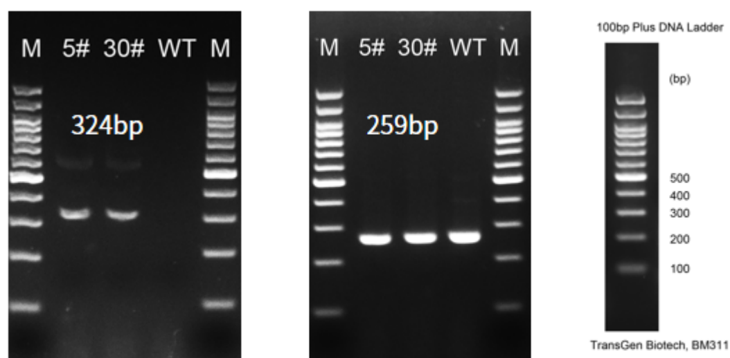
Fig1. Detection of DMPK expression in bladder by RT-PCR.
