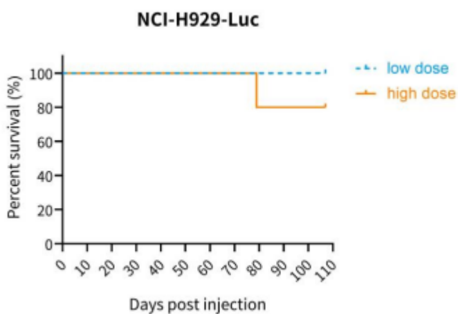
Figure 4. Survival curve of NCI-H929-Luc xenograft model (n=5)
